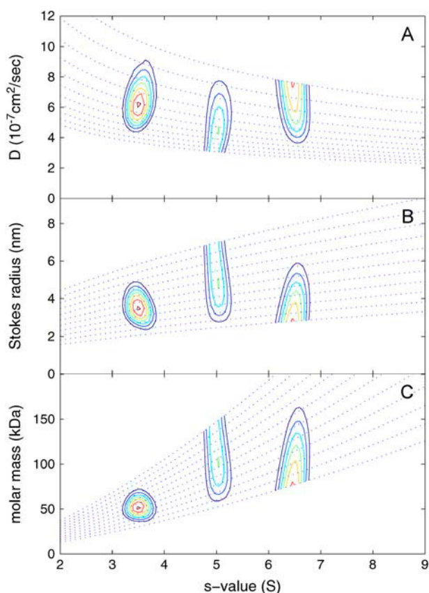
FIGURE 2 Contour plots of the transformation of c(s, f_r) from Fig. 1 to a c(s, D) distribution (A), a c(s, R_s) distribution (B), and a c(s, M) distribution (C). The dotted lines indicate lines of constant f_r . The distributions are not normalized (see Methods section).
