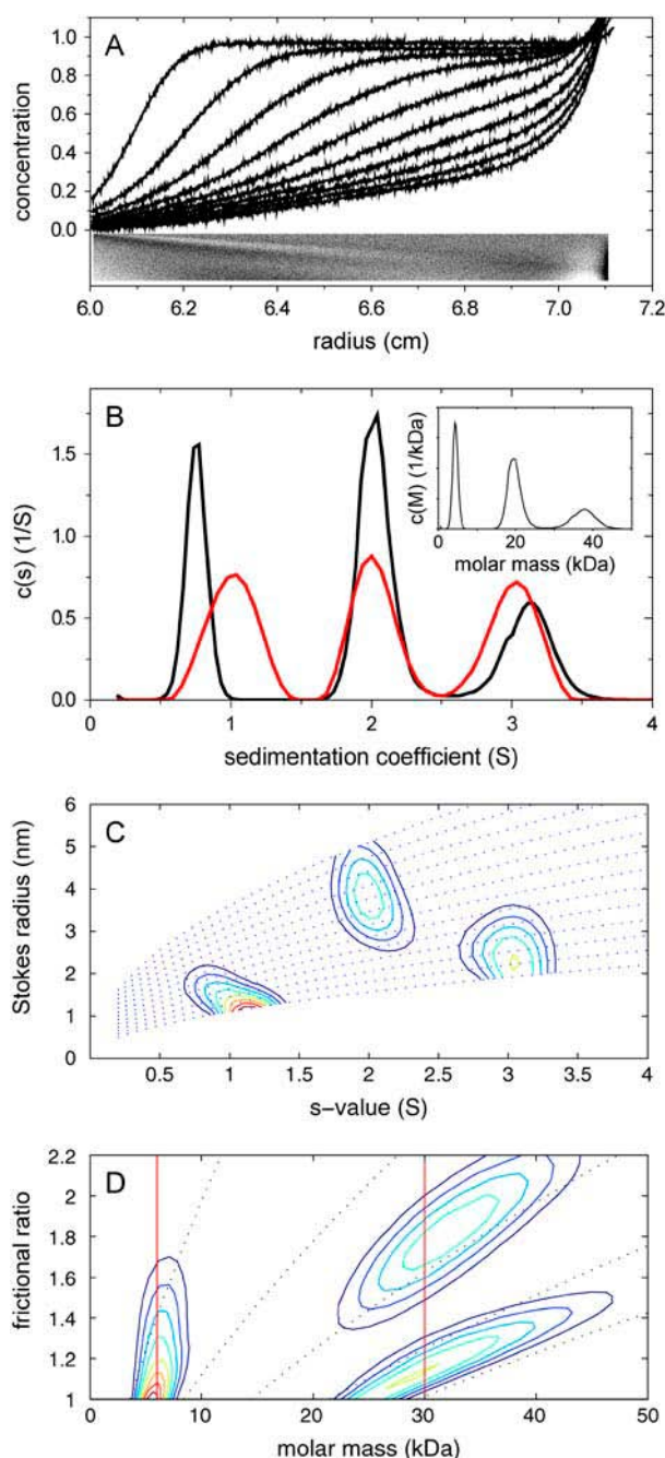
FIGURE 3 Application of c(s, f_r) analysis to a model system of small macromolecules. (A) Simulated signal profiles for a mixture of three species with 6 kDa, 1 S, 30 kDa, 2 S, and 30 kDa, 3 S, respectively, sedimenting at equal weight concentrations at a rotor speed of 50,000 rpm. Traces were calculated in time intervals of 600 s, for a period of 30,000 s, and 0.005 Gaussian noise was added. For clarity, only every fifth scan is shown. (B) c(s) analysis with maximum entropy regularization with P = 0.9 , with the corresponding c(M) distribution shown in the inset. The residuals bitmap of this fit is shown as an inset to panel A, scaled to \pm 0.02 black to white. Shown in red is the one-dimensional c(s, *) derived from the c(s, f_r) distribution by summation over all f_r -values for each s . (C and D) Calculated c(s, f_r) distribution, ranging from 0.2 to 4 S in 0.063 S steps, and from f_r = 1 –2.2 in 0.1 steps. Shown are the transformations as c(s, R_s) and c(s, M) , respectively. Also shown are lines of constant frictional ratio (dotted lines in C), and lines of constant s -value (dotted lines in D). The vertical red lines in panel D indicate the true molar mass values.
