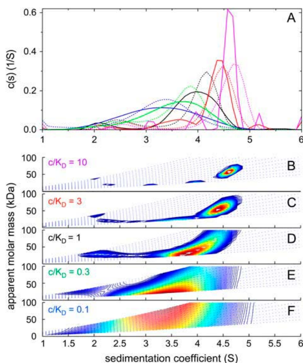
FIGURE 7 Application of c(s, f_r) to a reaction mixture with rapid kinetics on the timescale of sedimentation. Sedimentation velocity profiles were simulated for the interaction of a protein of 25 kDa, 2.5 S binding to a 40 kDa, 3.5 S species forming a 5 S complex with an equilibrium dissociation constant K_D = 3 \mu\text{M} , and a dissociation rate constant k_{\text{off}} = 0.01/\text{s} , studied at a rotor speed of 50,000 rpm. Interference optical detection was assumed, with conventional signal increments of 3.3 fringes/(mg/ml) and a noise level of 0.005 fringes. Concentrations were equimolar at 0.1-fold K_D (blue), 0.3-fold K_D (green), K_D (black), threefold K_D (red), and 10-fold K_D (magenta). c(s, f_r) distributions were calculated with s -values from 1 to 6 S and f_r -values from 0.8 to 2.0. Panel A shows c(s, *) distributions (solid lines) and conventional c(s) distributions (dotted lines), both normalized to constant area. Panels B–F show c(s, f_r) distributions mapped into the c(s, M) plane, at the concentrations indicated.
