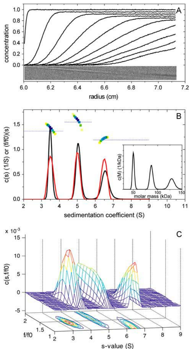
FIGURE 1 Application of c(s, f_r) analysis to a model system of large macromolecules. (A) Simulated signal profiles for a mixture of three species with 50 kDa, 3.5 S, 100 kDa, 5 S, and 100 kDa, 6.5 S, respectively, loaded at equal weight concentrations in a solution column from 6.0 to 7.2 cm, and sedimenting at a rotor speed of 50,000 rpm at 20°C. Traces were calculated in time intervals of 300 s, for a period of 15,000 s, and 0.005 Gaussian noise was added. For clarity, only every fifth scan is shown. (B) c(s) analysis with maximum entropy regularization with P = 0.7 (black line). The transformation of c(s) to c(M) is shown in the inset. The residuals bitmap of this fit is shown as inset to panel A, scaled to \pm 0.02 black to white. Shown in red in panel B is the c(s, *) distribution derived from the c(s, f_r) distribution by summation over all f_r -values. The colored squares are the weight-average f_r -values for each s -value from c(s, f_r) distribution, with the color density indicating the signal at each s -value. The blue dotted horizontal lines are the weight-average frictional ratios for a conventional, but segmented c(s) model with one segment for each peak. (C) The calculated c(s, f_r) distribution is shown as two-dimensional distribution with grid lines representing the s and f_r grid of the analysis. Below this c(s, f_r) surface is shown a contour plot of the distribution projected into the s - f_r plane, where the magnitude of c(s, f_r) is indicated by contour lines at constant c(s, f_r) in equidistant intervals of c .
