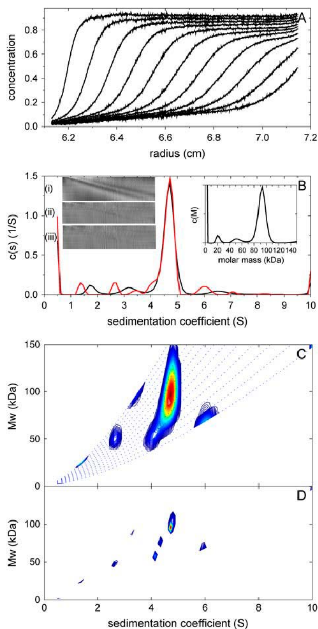
FIGURE 5 Analysis of experimental sedimentation velocity data from the study of the oligomeric state of a glycosylated NK receptor fragment. For experimental details, see Dam and Schuck (28). Panel A shows a representative subset of the raw data. Panel B shows c(s) analysis (black line) and transformation to c(M) (right inset). The left insets are residual bitmaps from (i) a single discrete species analysis, (ii) the c(s) analysis, and (iii) the c(s, f_r) analysis. The red line is the c(s, *) trace of the c(s, f_r) distribution shown in panel C. Panel D shows the same analysis as in panel C, but without regularization.
