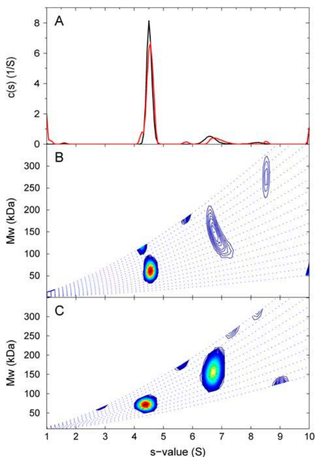
FIGURE 6 Analysis of SV data from a bovine serum albumin sample (commercial sample used without further purification) sedimenting at 55,000 rpm, 22°C. Panel A shows c(s) distribution (black) and c(s,*) distribution (red) derived from the c(s, f_r) fit shown in panel B as c(s, M) . Integration of the c(s, f_r) peak results in an average apparent molar mass of 61 kDa (assuming a \bar{v} value of 0.73 ml/g) for the monomer at \sim 4.5 S, and 135 kDa for the dimer peak at \sim 7 S, which amounts to \sim 9\% of the total sedimenting material. The dotted lines are lines of constant f_r . Panel C shows analysis of a mixture of a bovine serum albumin (taken from a different batch) with an IgG sample, sedimenting at 50,000 rpm, 20°C. Integration of the IgG peak leads to an average apparent molar mass of 154 kDa (assuming a \bar{v} value of 0.73 ml/g).
