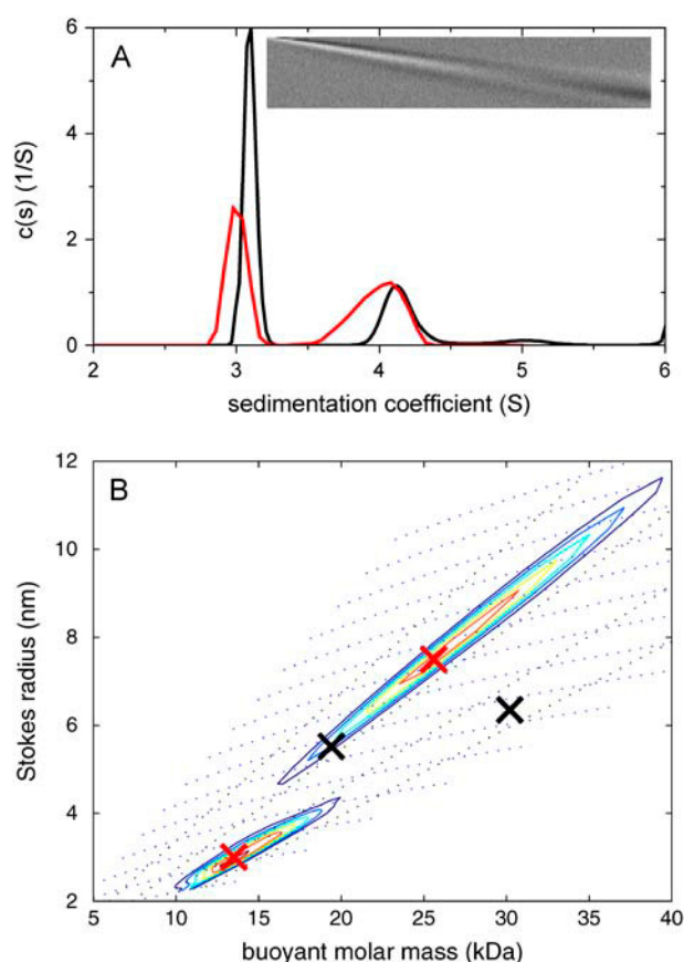
FIGURE 4 Analysis of a theoretical mixture of two species with buoyant molar mass of 25.6 kDa and 3 S (corresponding, for example, to 160 kDa extended polymer with \bar{v} = 0.84 ml/g), and with buoyant molar mass 13.5 kDa and 4 S (corresponding, for example, to a folded protein of 50 kDa). Sedimentation was simulated under the same conditions as in Figs. 1 and 3. (A) The c(s) distribution is shown as a black line, with the residuals bitmap from the c(s) analysis in the inset ( \text{rmsd} = 0.0074 ). The red line is the c(s, *) trace from the c(s, f_r) analysis, which is shown in panel B as a transformation to a parameter space of buoyant molar mass and Stokes radius. The dotted lines indicate directions of constant f_r and constant s . The red crosses are the parameters underlying the simulation, the black crosses are values resulting from integration of an impostor c(M) transformation of c(s) .
